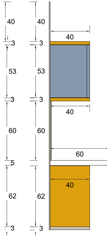
SIDE ELVATION
