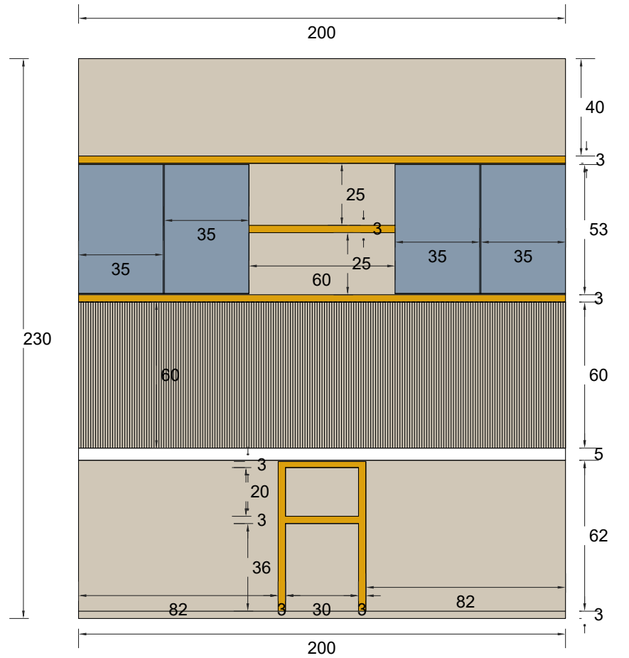
STUDY FRONT ELEVATION
